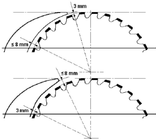
Adjusting the riving knife
