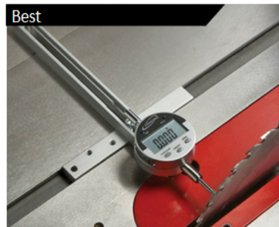
A dedicated saw dial indicator. Such as this one by 'lgaging'
